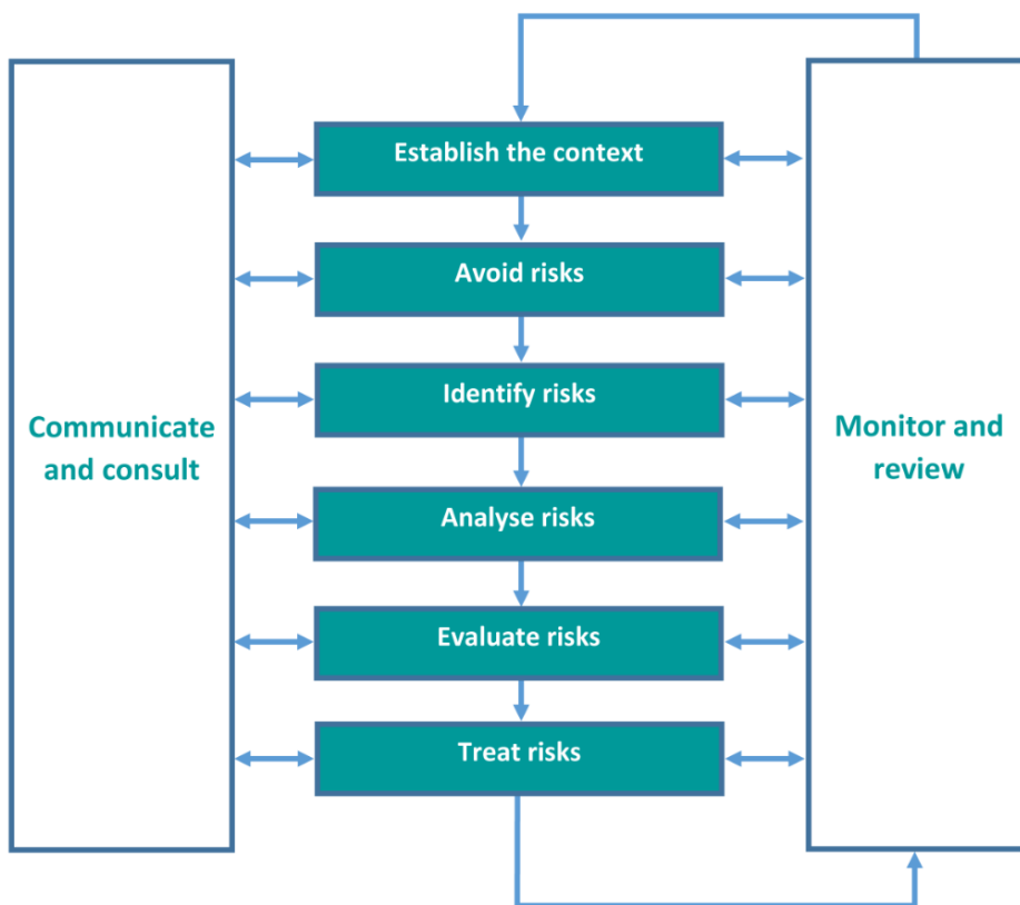
Figure 3. Risk management
